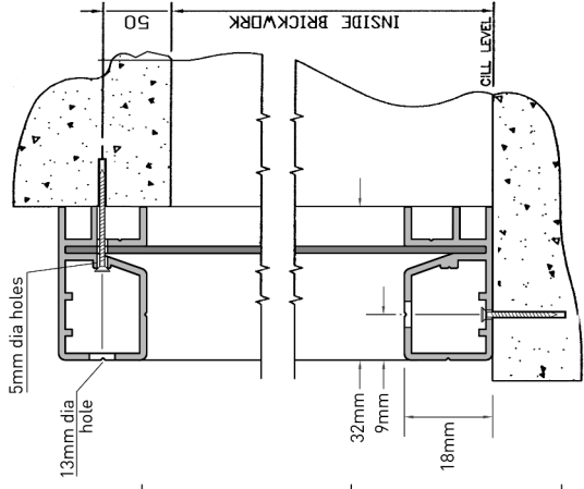
SECTION A-A FULL SIZE
