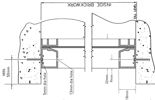
SECTION A-A FULL SIZE
