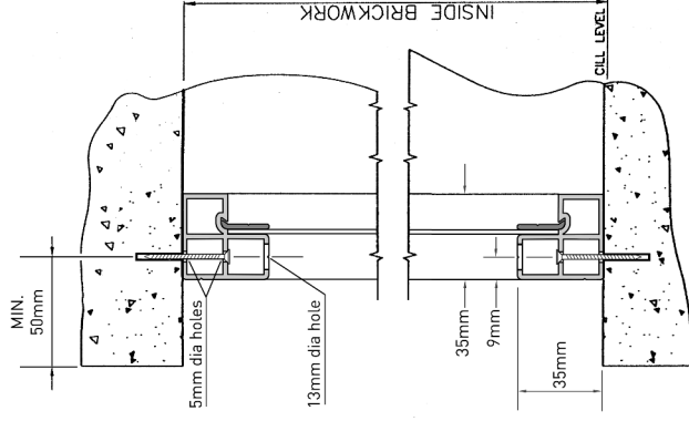
SECTION A-A FULL SIZE
